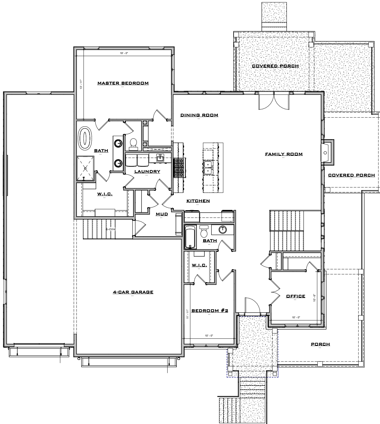
OLYMPIC MAIN LEVEL FLOOR PLAN
