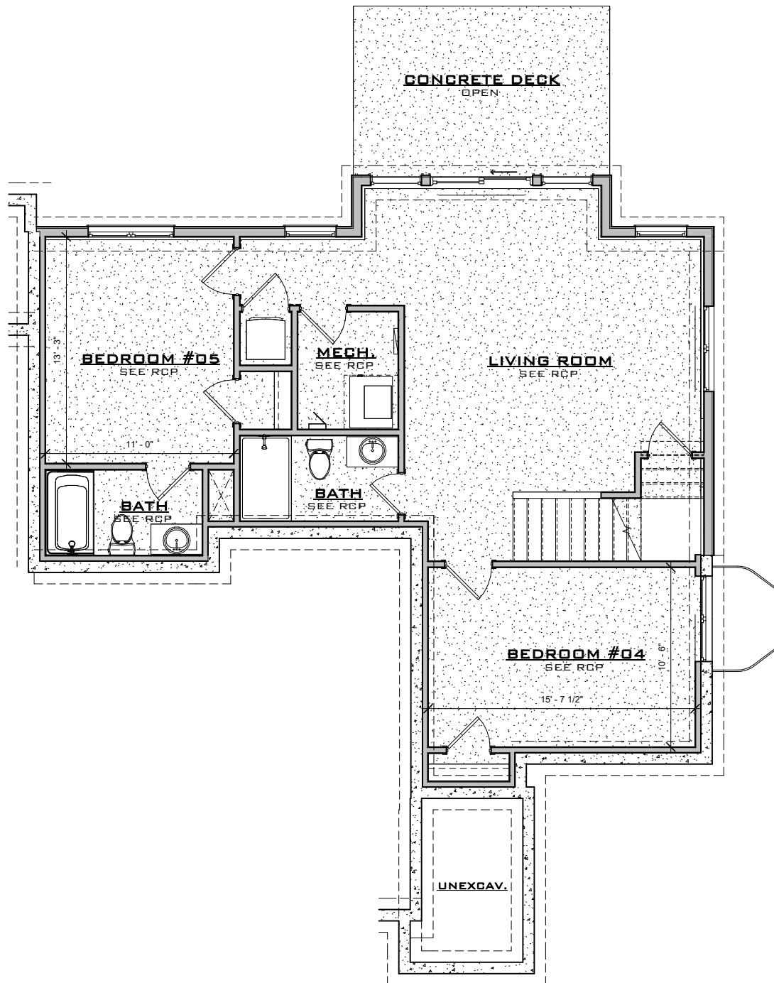
HAWTHORNE BASEMENT LEVEL PLAN
