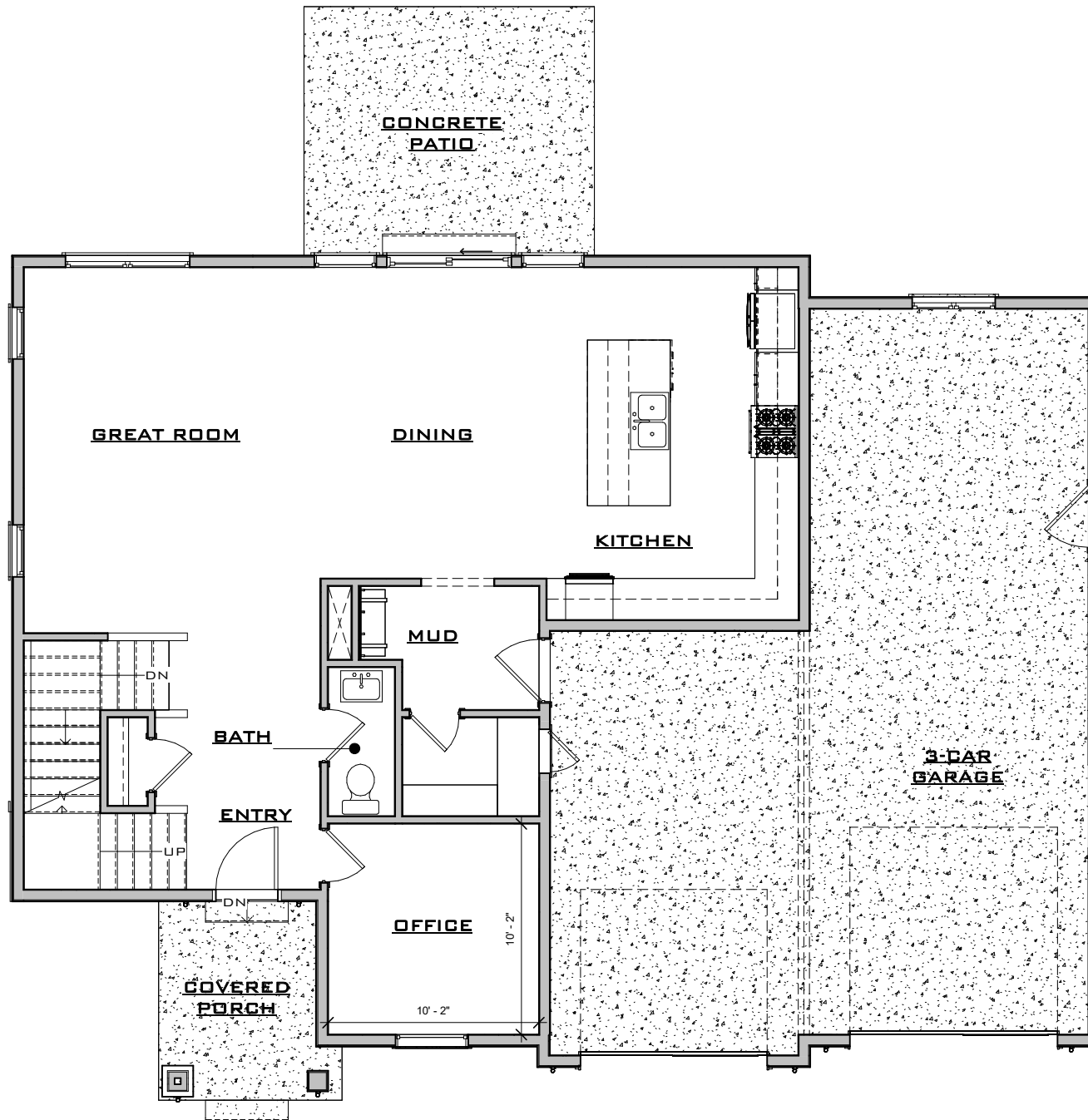
DURIAN MAIN LEVEL FLOOR PLAN
