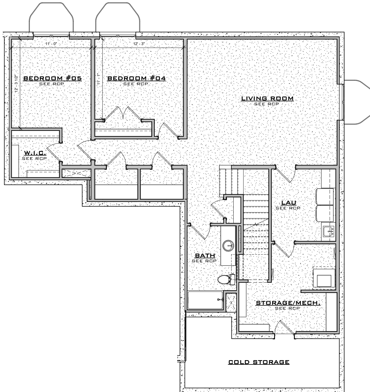
MAGNOLIA BASEMENT LEVEL FLOOR PLAN
