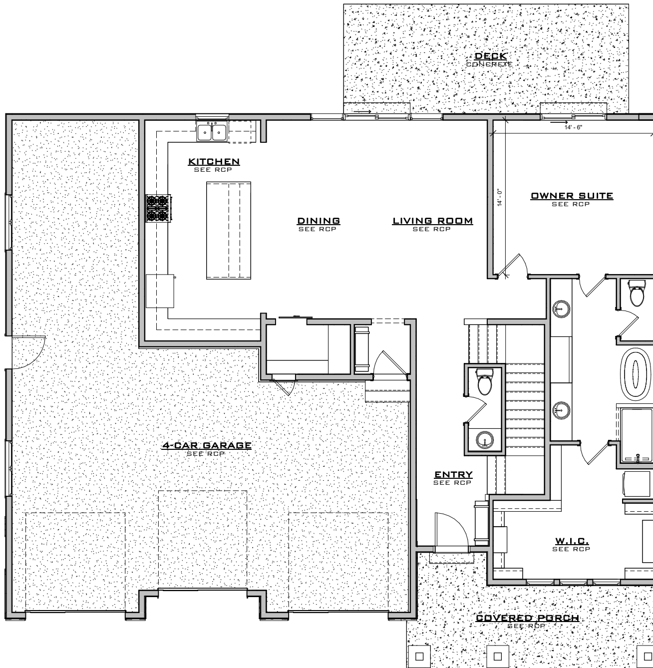
MAGNOLIA MAIN LEVEL FLOOR PLAN
