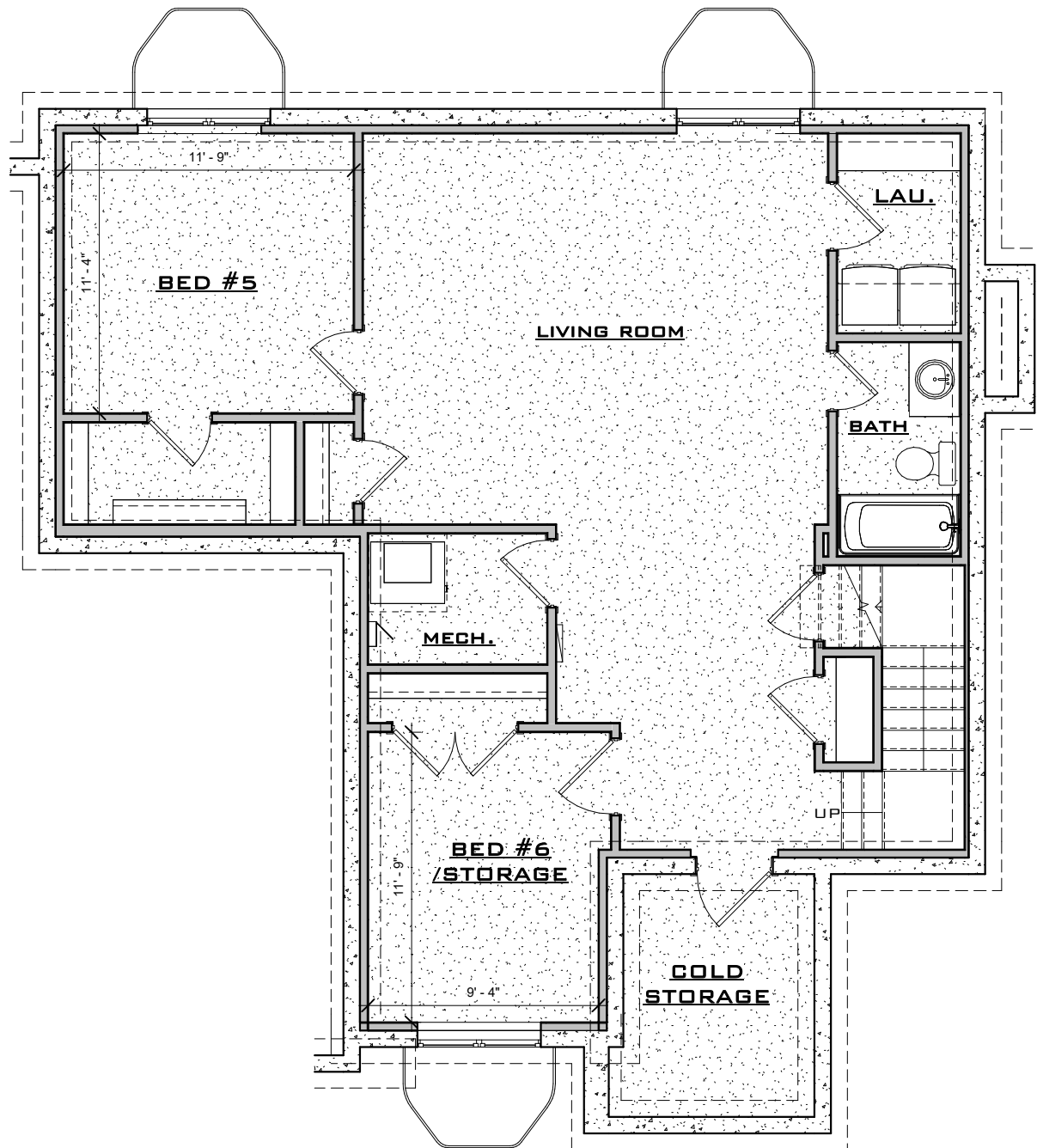
DURIAN BASEMENT FLOOR PLAN
