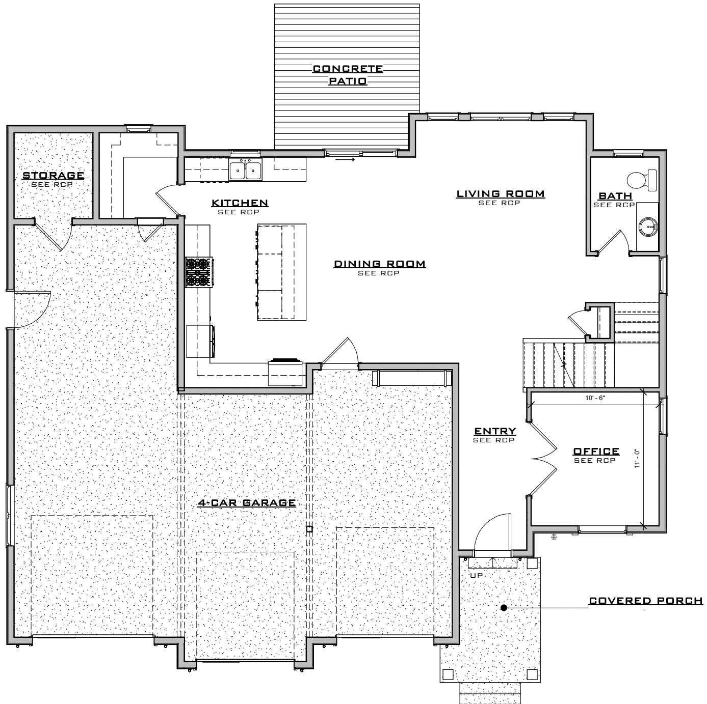
HAWTHORNE MAIN LEVEL FLOOR PLAN
