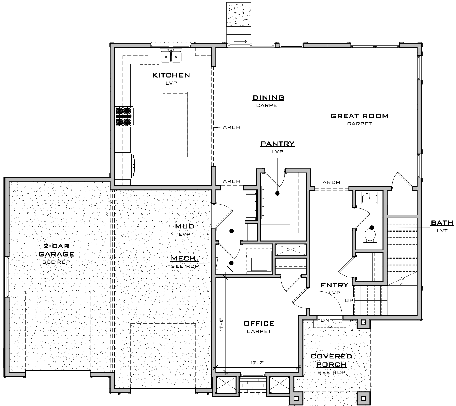
YARROW MAIN LEVEL FLOOR PLAN
