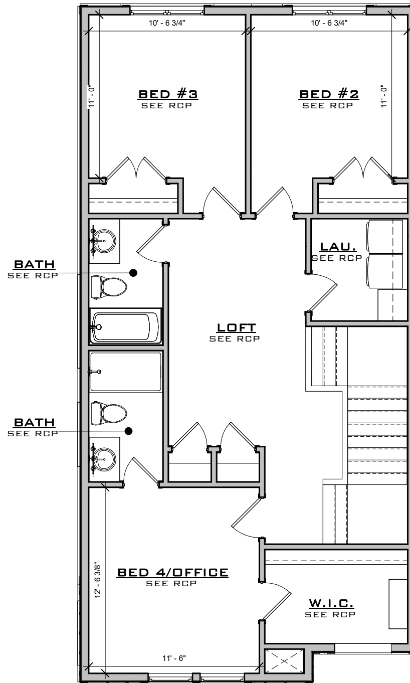
POPPY SECOND LEVEL FLOOR PLAN
