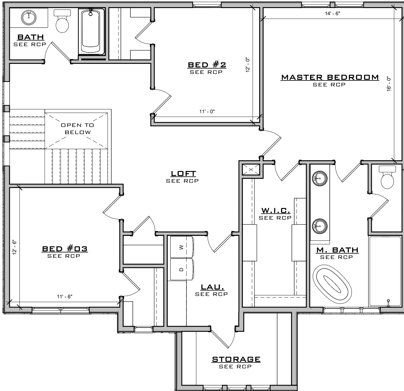
SECOND LEVEL FLOOR PLAN
