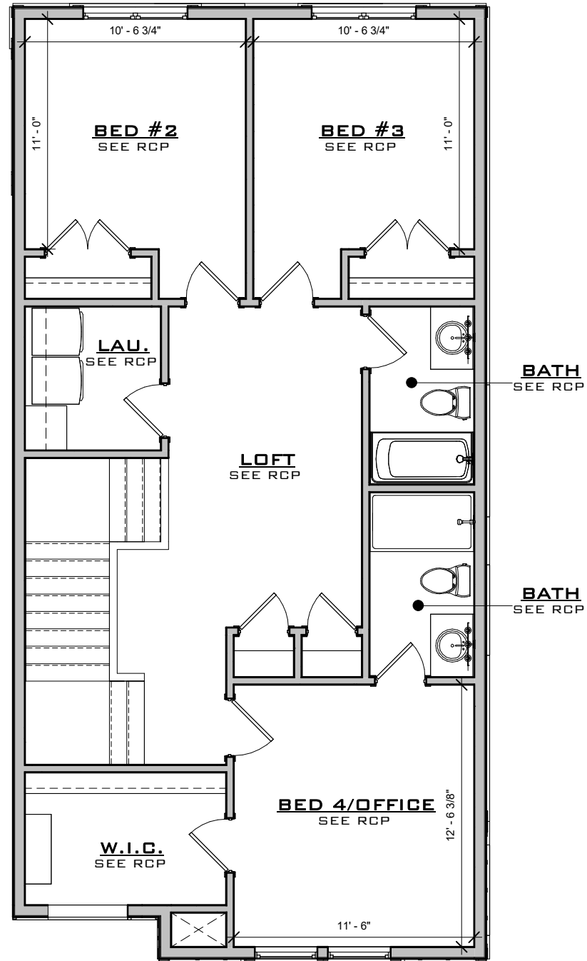
POPPY SECOND LEVEL FLOOR PLAN
