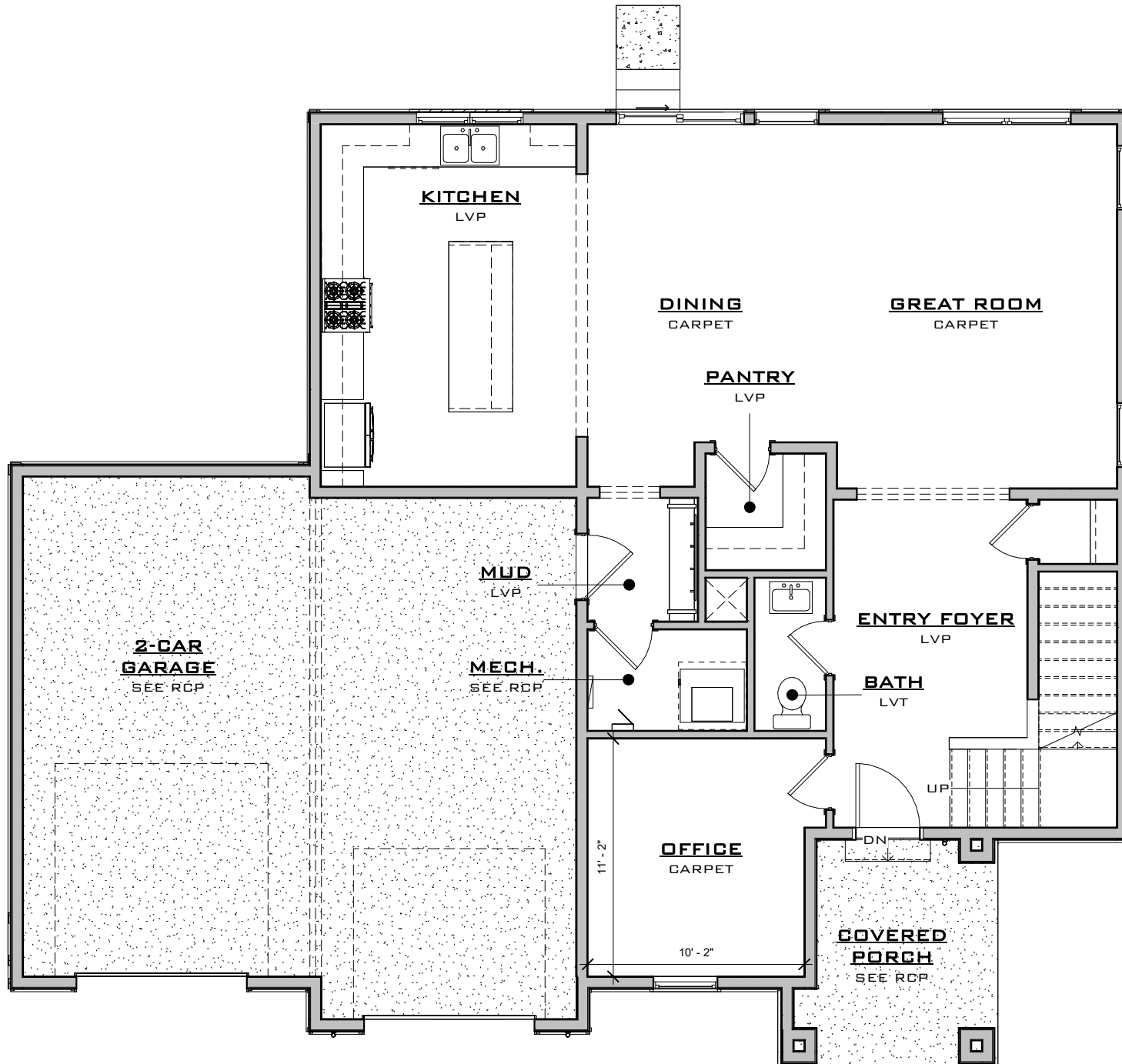
YARROW MAIN LEVEL FLOOR PLAN
