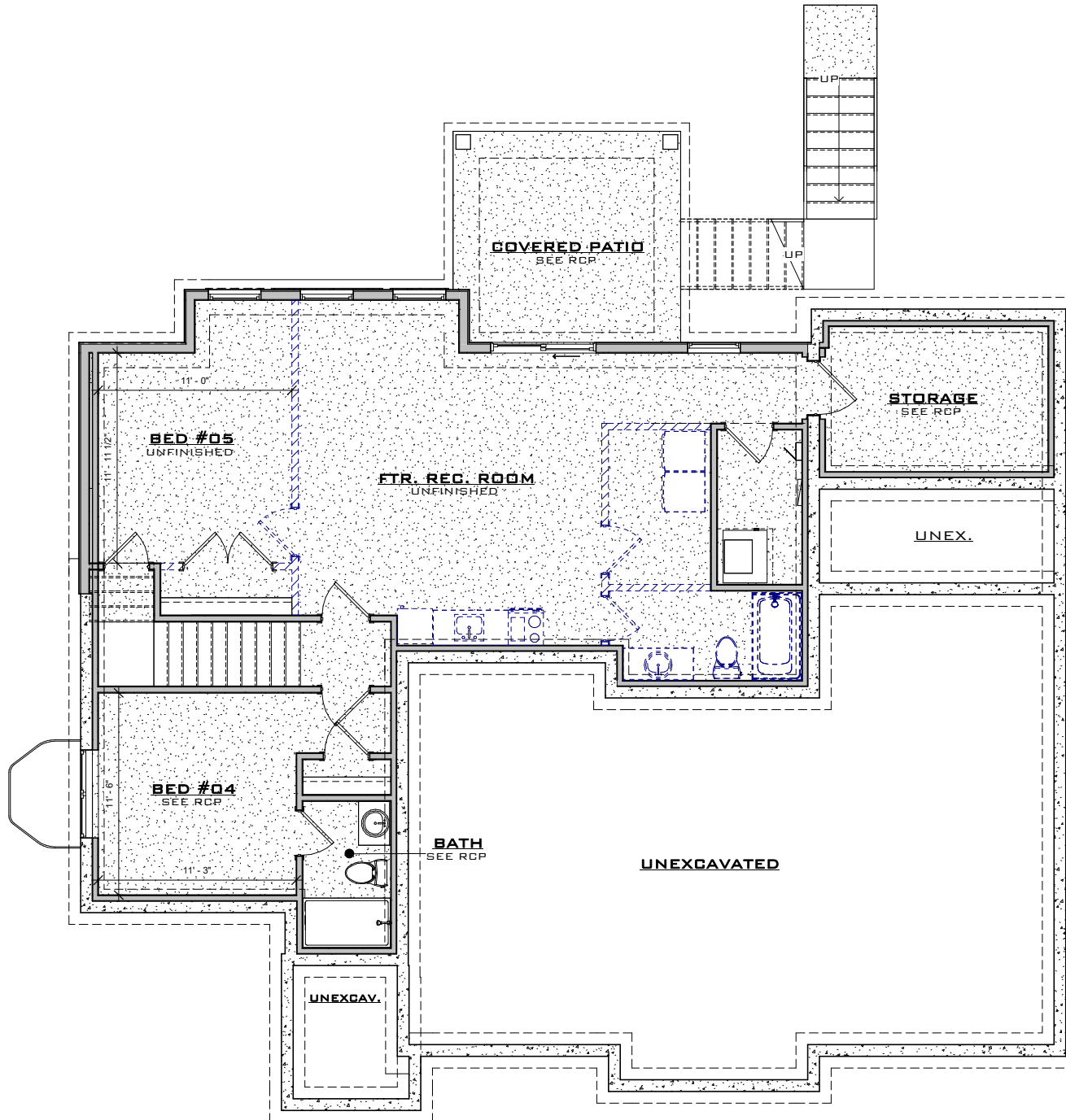
HAWTHORNE BASEMENT LEVEL FLOOR PLAN
