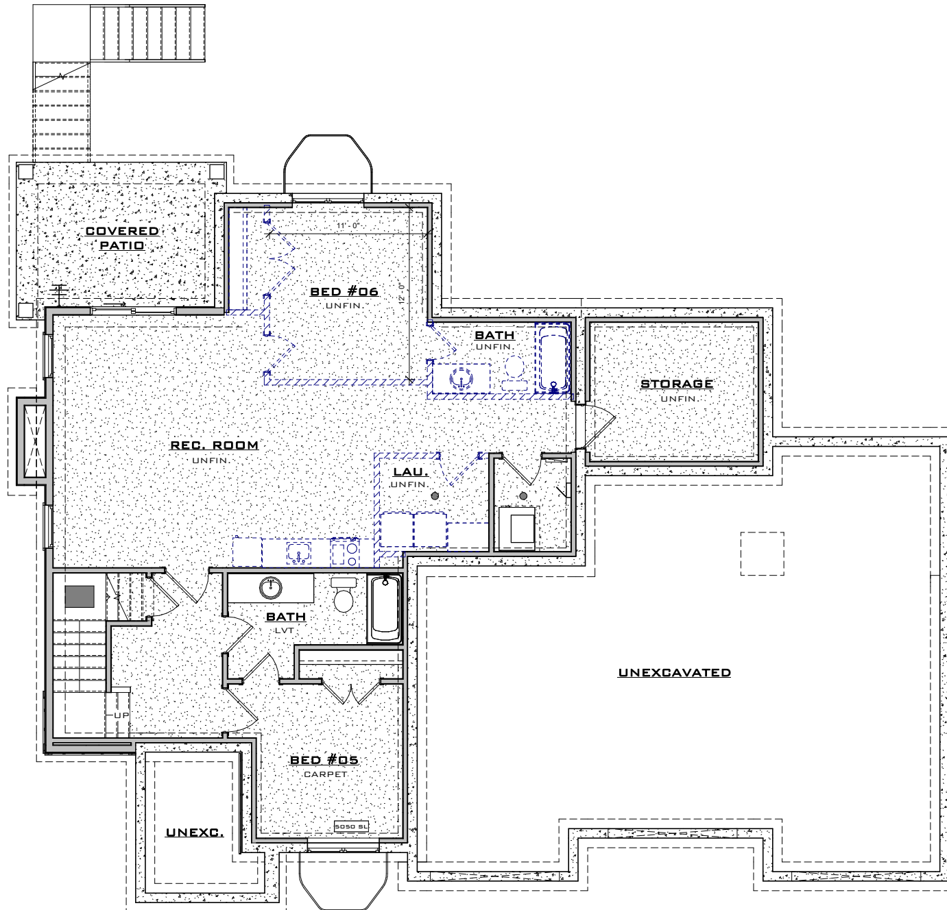
BASEMENT LEVEL FLOOR PLAN
