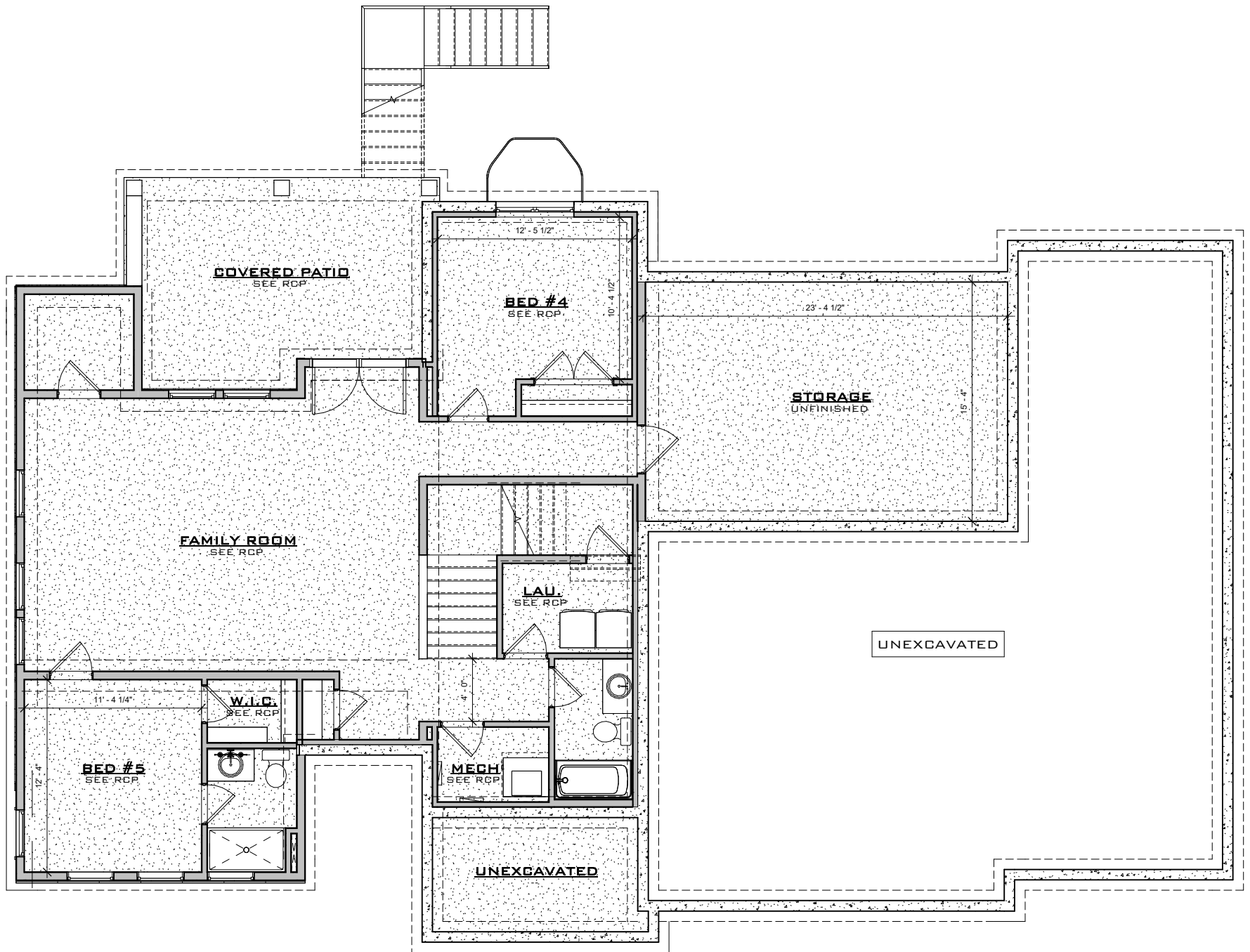
SEQUOIA BASEMENT FLOOR PLAN
