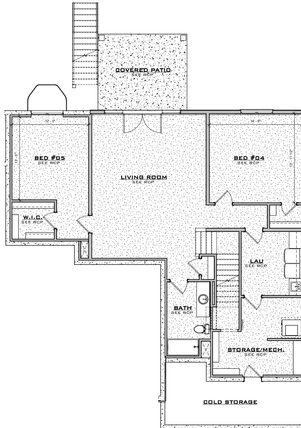
MAGNOLIA BASEMENT LEVEL FLOOR PLAN
